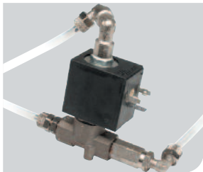
Mixer solenoid valve guarantees instant beverages with optimal differentiated temperatures
